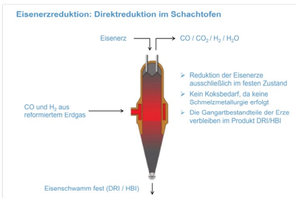
Direct reduction in the shaft furnace.
