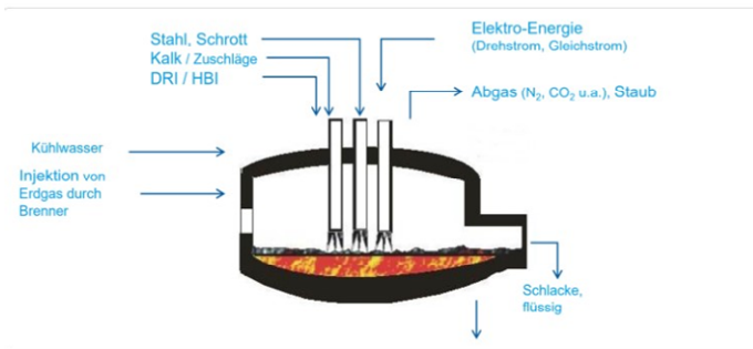
Crude steel production in electric arc furnace.
